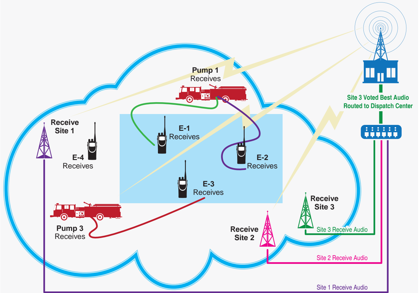
The dispatch center's high-power transmitter allows all radios on the fireground to receive.
